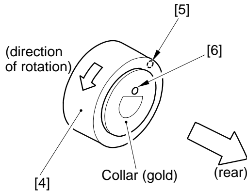
Figure 2-23 Pick-Up Roller for the Rear
