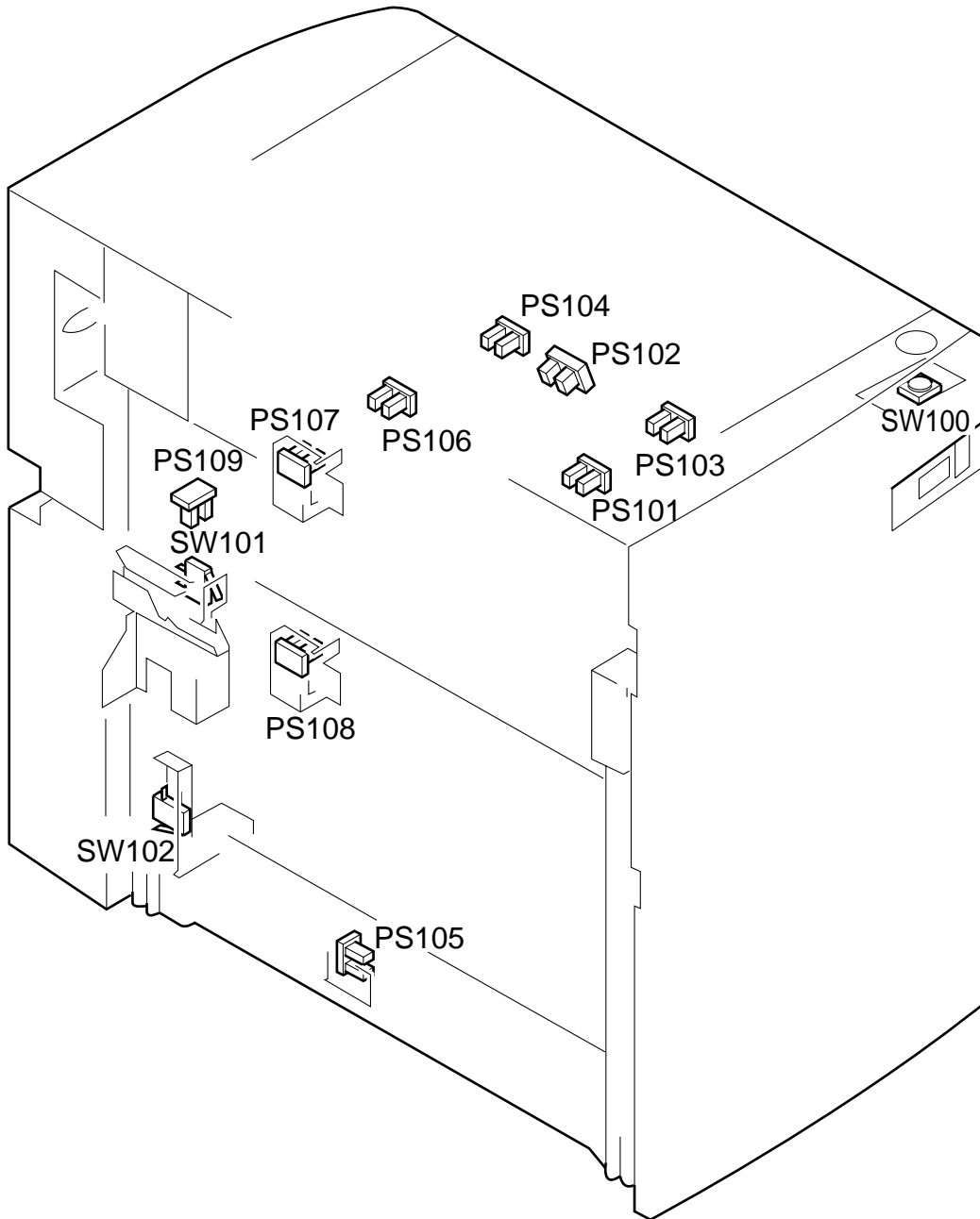
Figure 3-7a (side paper deck)
