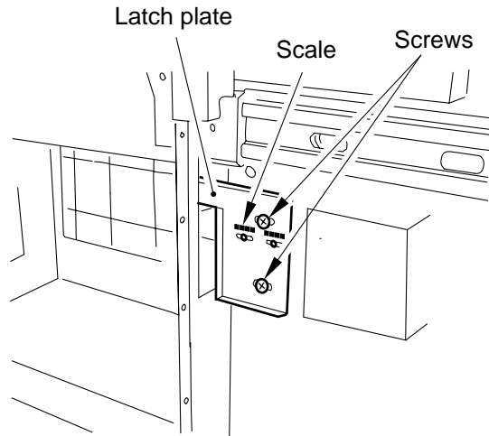
Figure 2-7 (rear left of the compartment)
