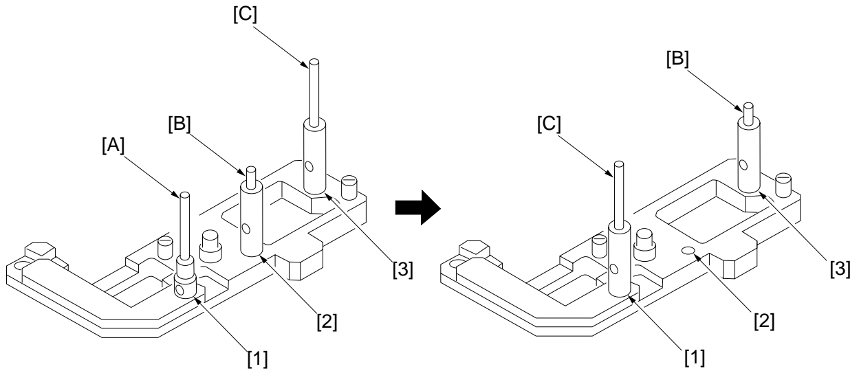
FY9-3009-040 Before Repositioning the Pins
